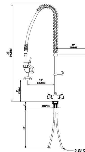
JC-300B 台式双温 Desk-mounted double temperature
