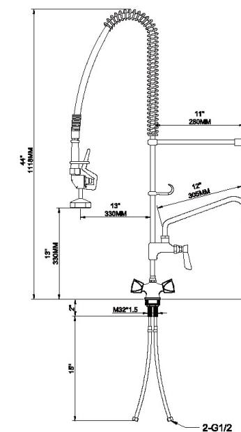
JC-300B-A 台式双温 Desk-mounted double temperature
